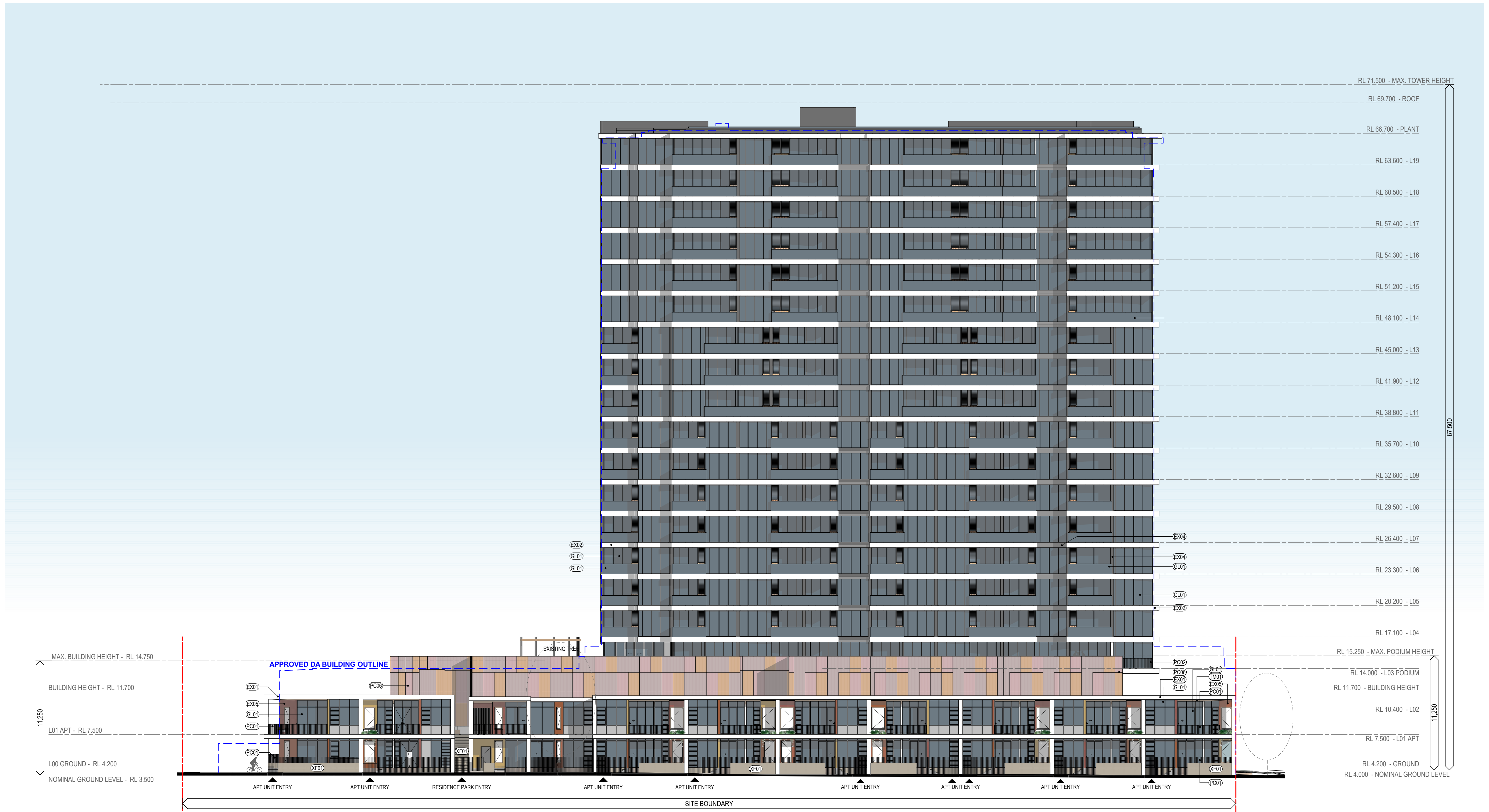
1 SD ELEVATION - NORTH SCALE 1:200 @ A1 SCALE 1:400 @ A3
