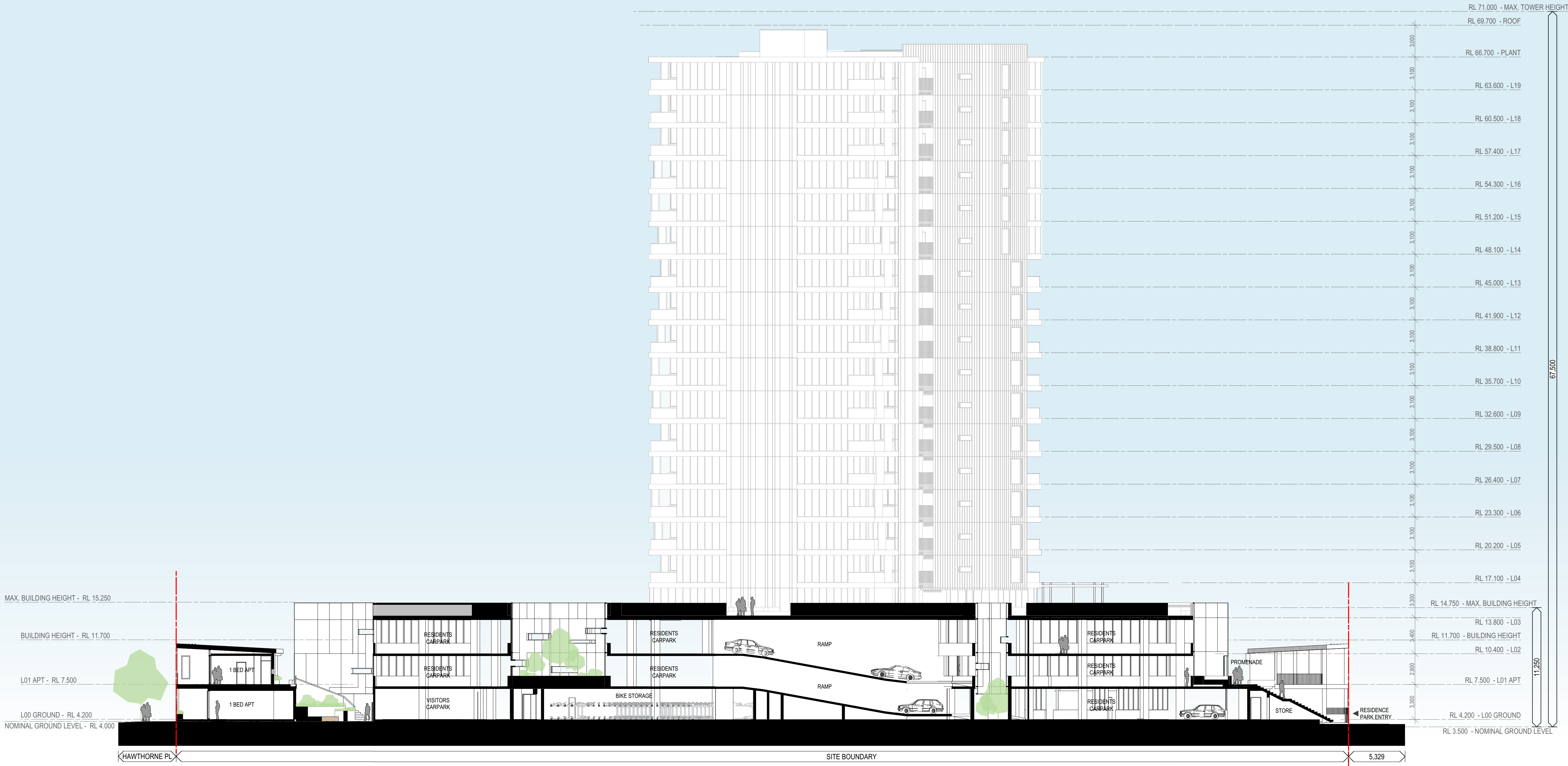
3 - 04 SECTION (01) SCALE 1:200 @ A1 SCALE 1:400 @ A3
