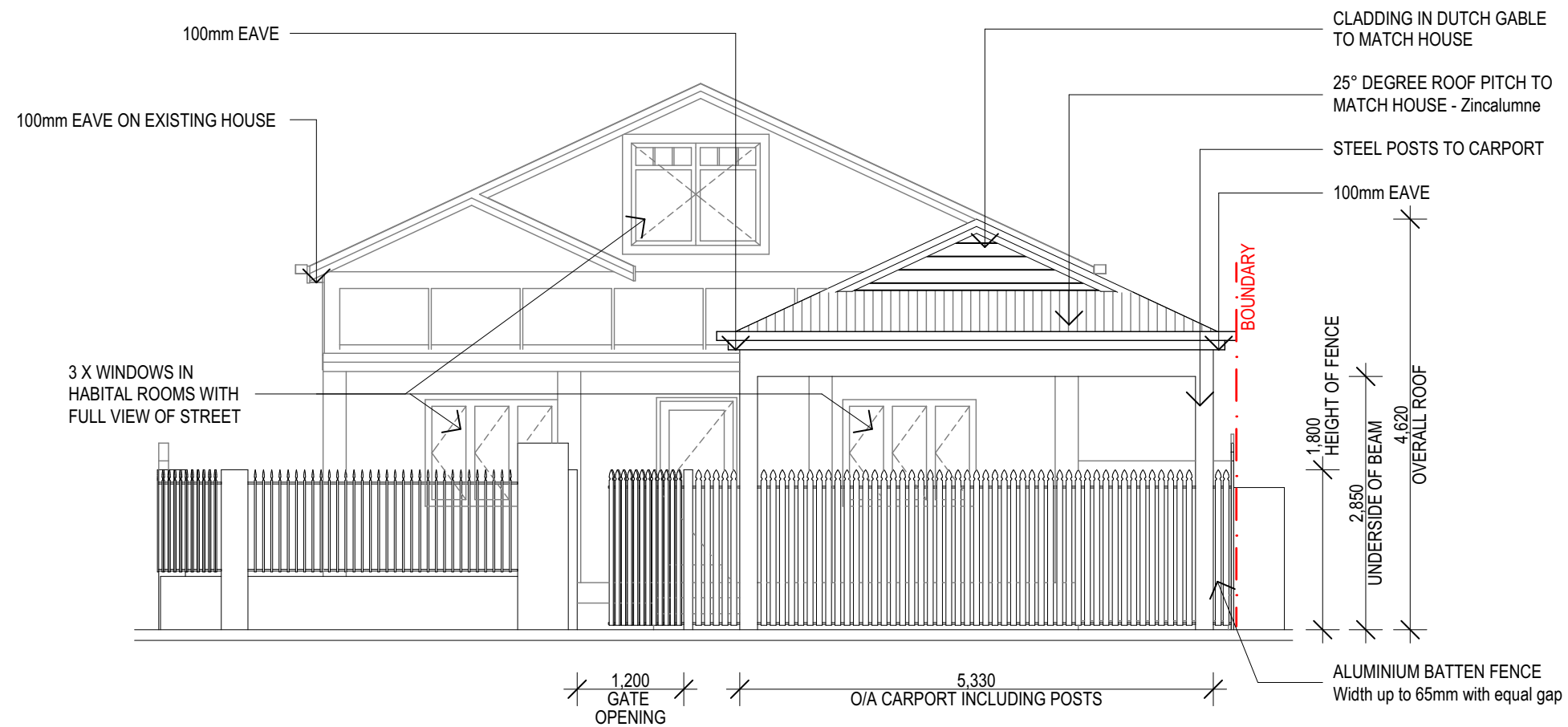
01 FRONT ELEVATION
