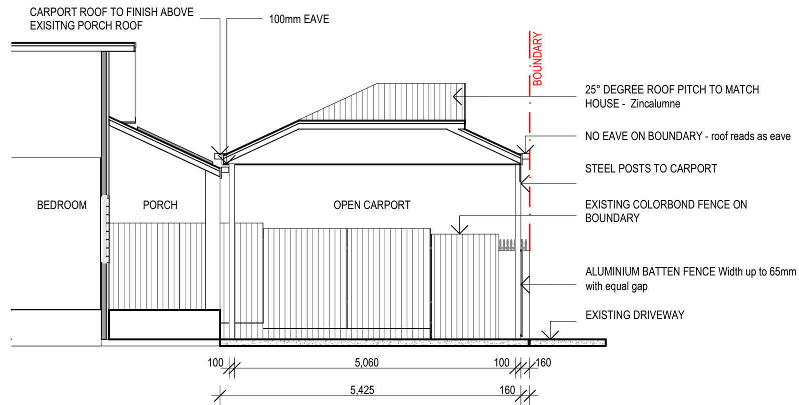
02 SECTION
